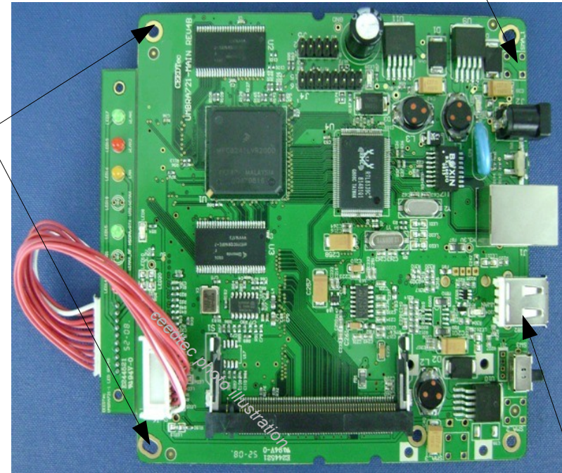
USB2.0 Host I/F
